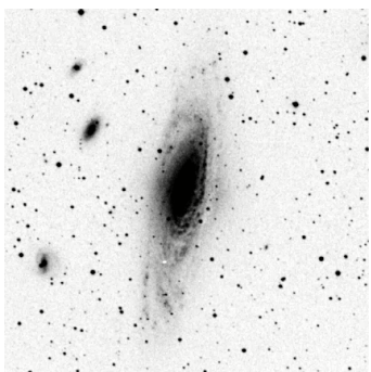
NGC7331 Gal. 12.0'
