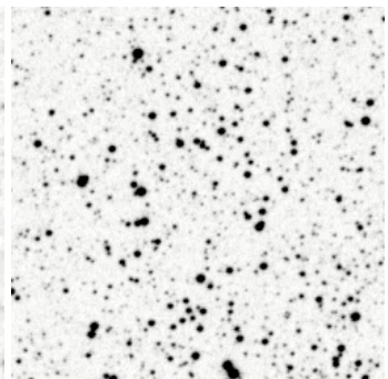
NGC6645 O.C. 7.0'
