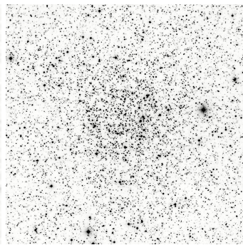
NGC7789 O.C. 30.0'
