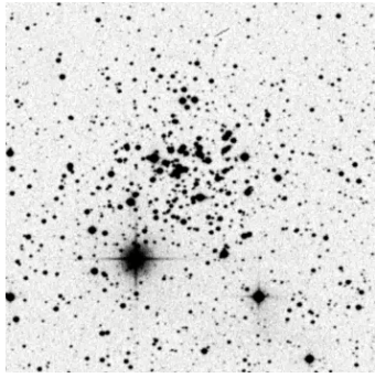
NGC654 O.C. 10.0'
