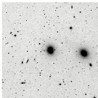
NGC7626/Peg-Clstr. Gal. 20.0'
