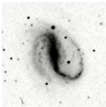
NGC7479 Gal. 5.0'
