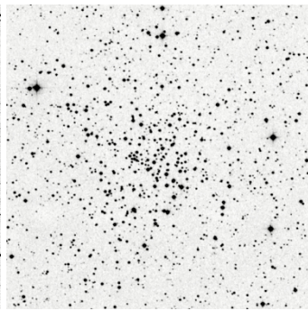
NGC6939 O.C. 15.0'
