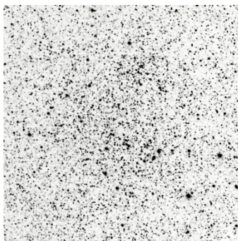
NGC6755 O.C. 20.0'
