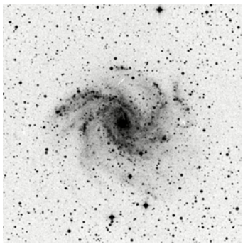
NGC6946 Gal. 15.0'
