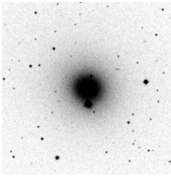
NGC5846 Gal. 10.0'
