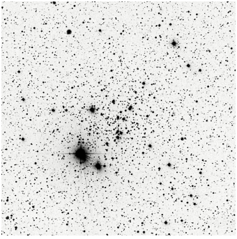
NGC457 O.C. 30.0'
