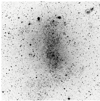
NGC6822 Gal. 15.0'
