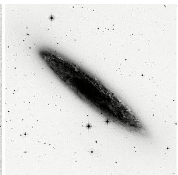
NGC253 Gal. 30.0'
