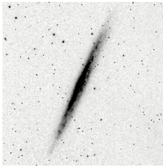
NGC5907 Gal. 10.0'
